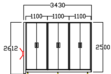
FRONT VIEW COMPACTOR LAST UNIT DFM 21 ( UNIT 1) DFM 13 (UNIT 2)
