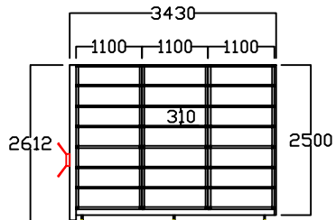
FRONT VIEW COMPACTOR UNIT 1 AND UNIT 2 IN OPEN CONDITION
