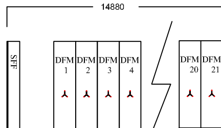
SIDE VIEW COMPACTOR UNIT 1
